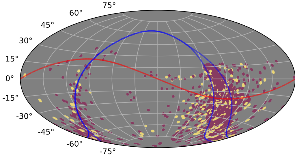
mw_roll_bulge_v3.3_10yrs : XRBPopMetric_early_detect
