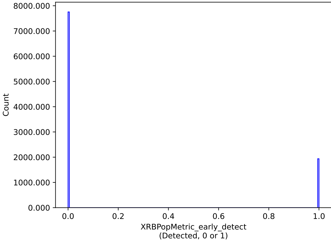
mw_roll_bulge_v3.3_10yrs : XRBPoMetric_early_detect
