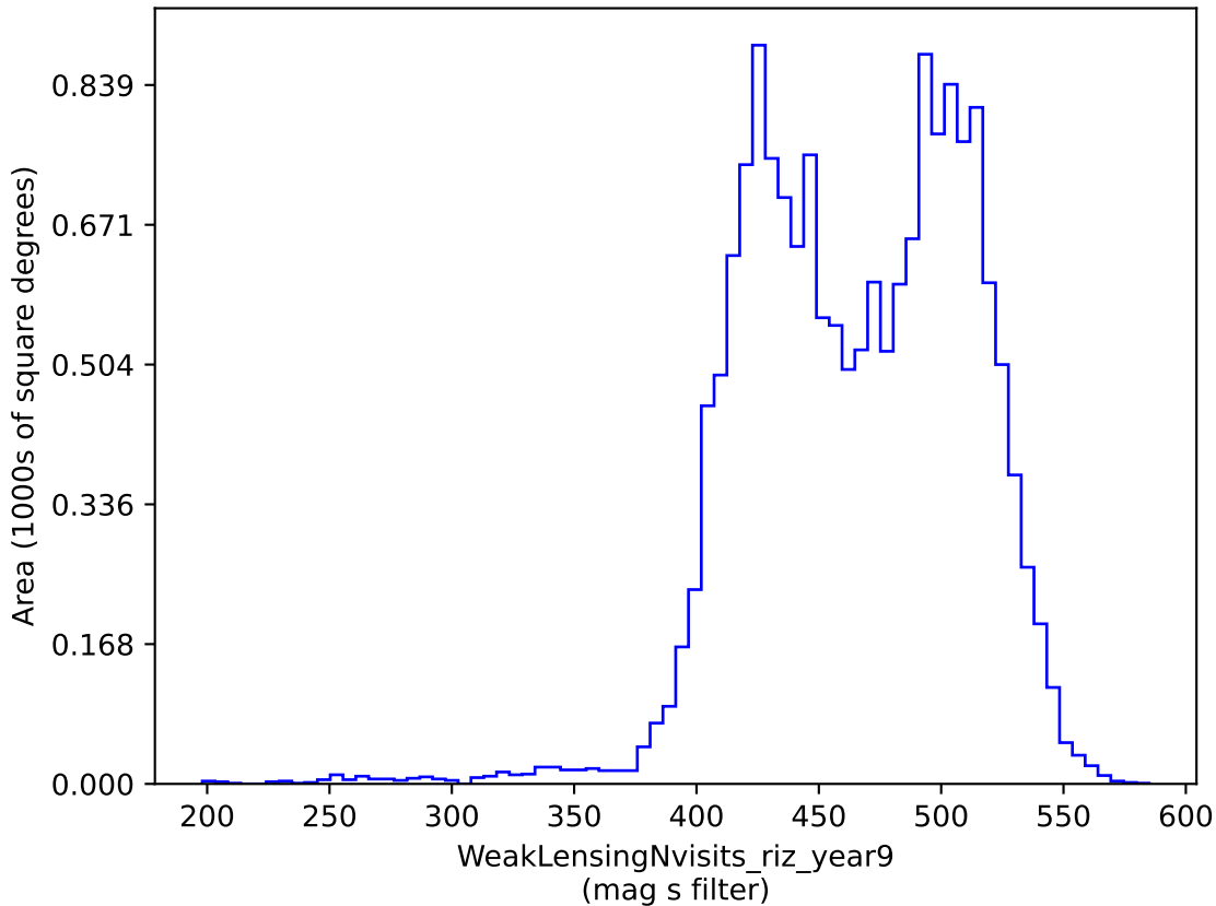
mw_roll_bulge_v3.3_10yrs gri band non-DD: WeakLensingNvisits_riz_year9
