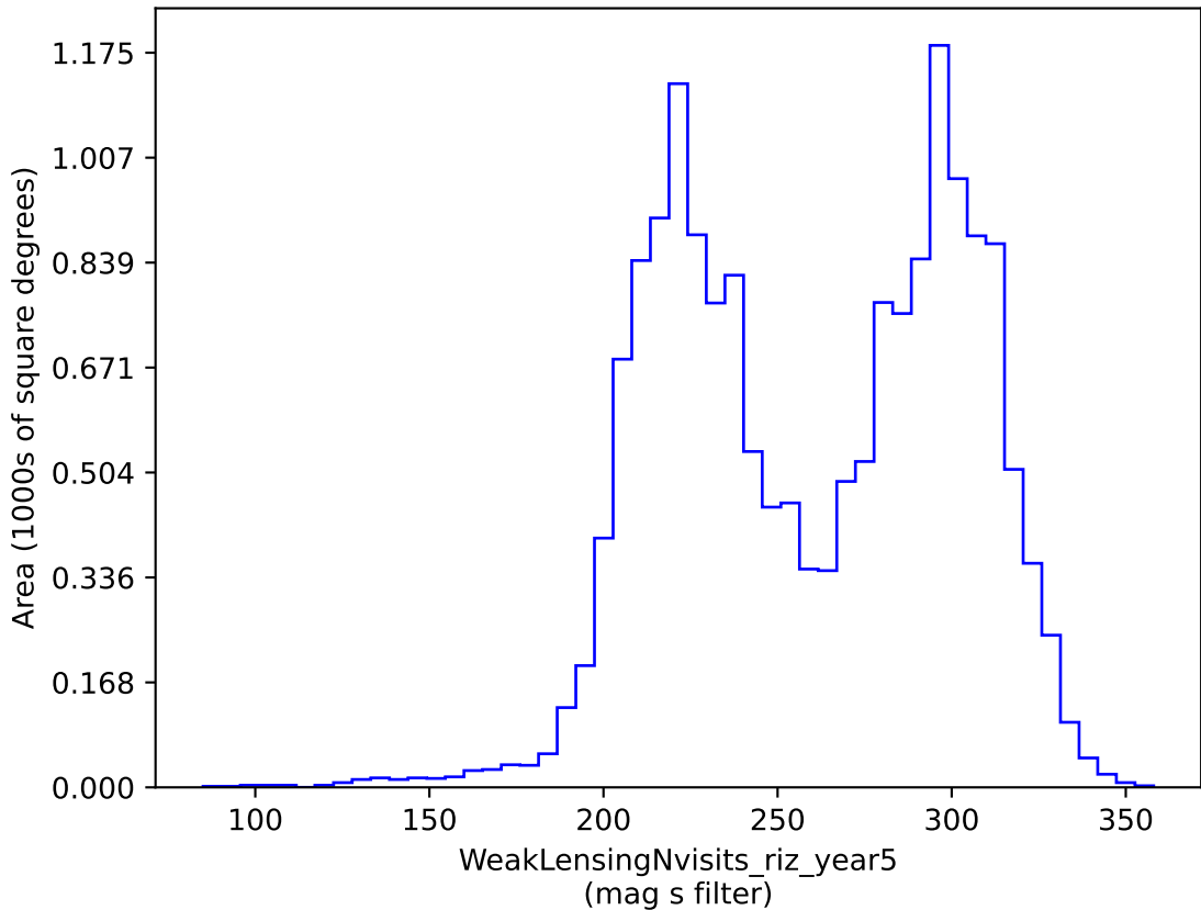
mw_roll_bulge_v3.3_10yrs gri band non-DD: WeakLensingNvisits_riz_year5
