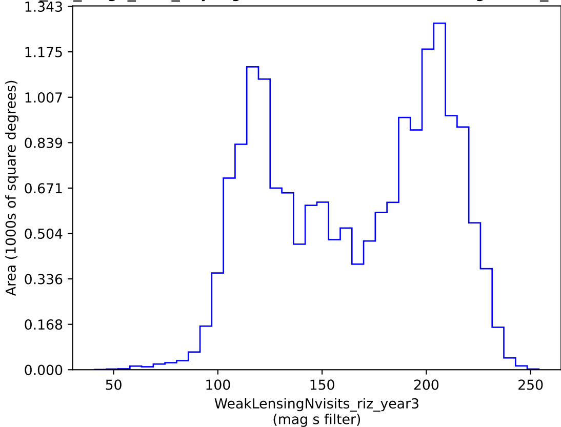
mw_roll_bulge_v3.3_10yrs gri band non-DD: WeakLensingNvisits_riz_year3
