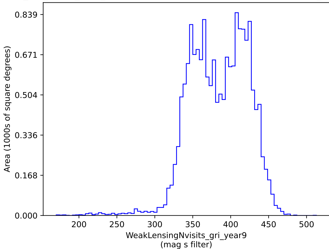
mw_roll_bulge_v3.3_10yrs gri band non-DD: WeakLensingNvisits_gri_year9
