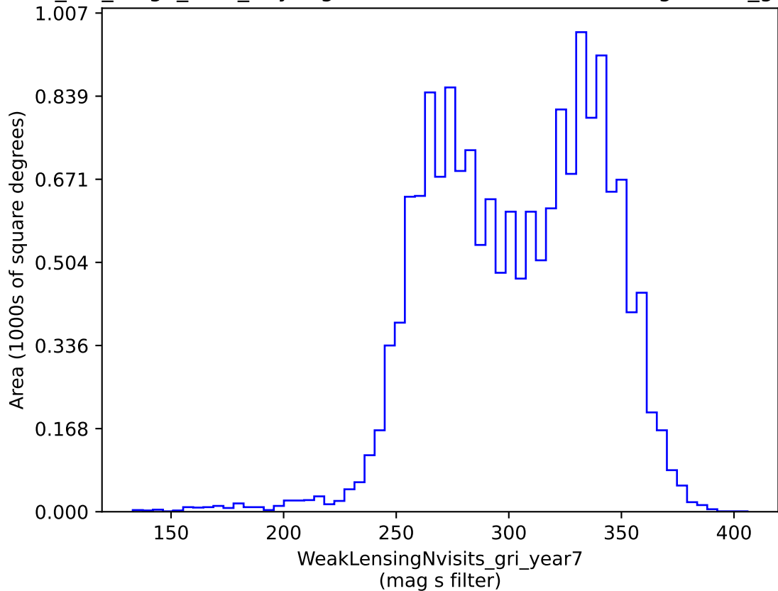
mw_roll_bulge_v3.3_10yrs gri band non-DD: WeakLensingNvisits_gri_year7
