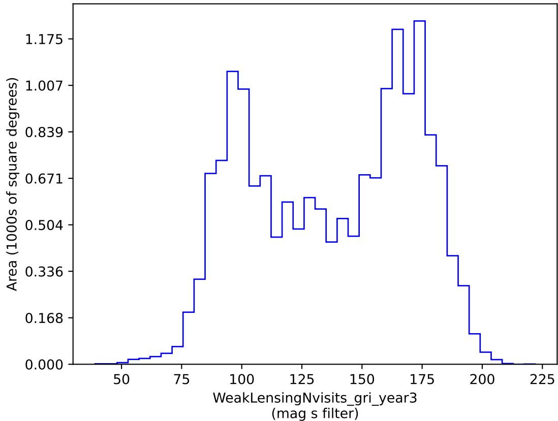
mw_roll_bulge_v3.3_10yrs gri band non-DD: WeakLensingNvisits_gri_year3
