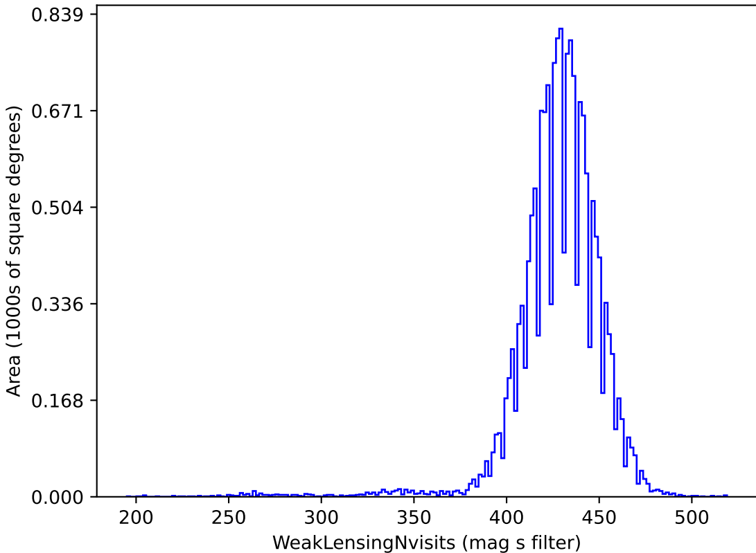
mw_roll_bulge_v3.3_10yrs gri band non-DD: WeakLensingNvisits
