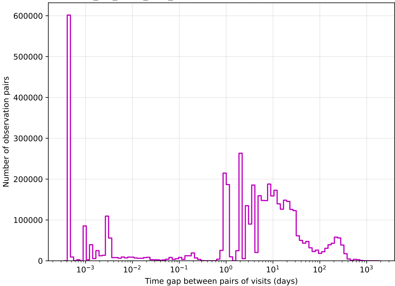
mw_roll_bulge_v3.3_10yrs z band: Tgaps observationStartMJD
