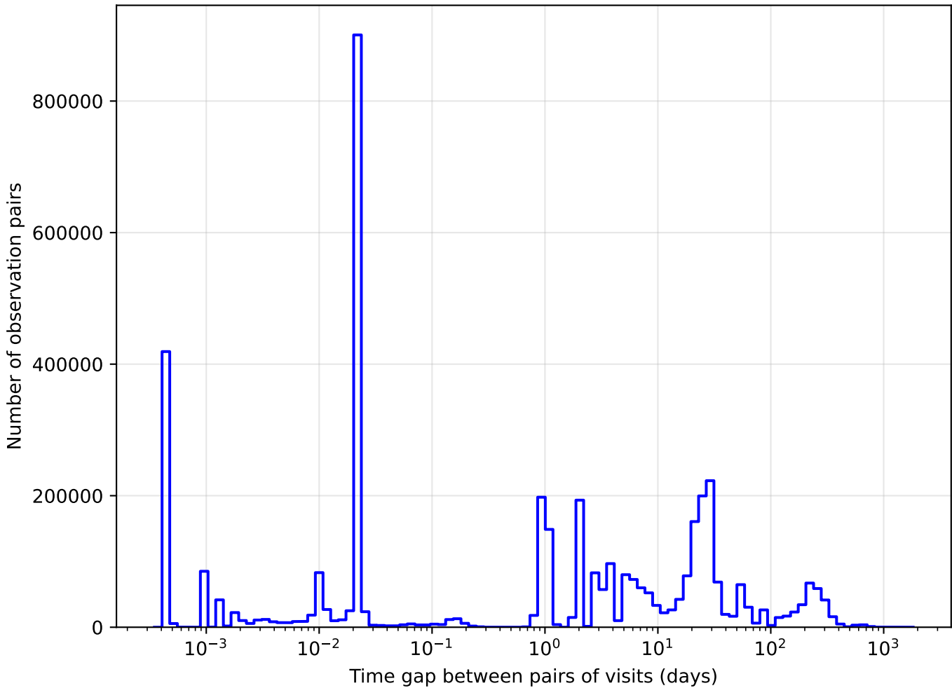
mw_roll_bulge_v3.3_10yrs y band: Tgaps observationStartMJD
