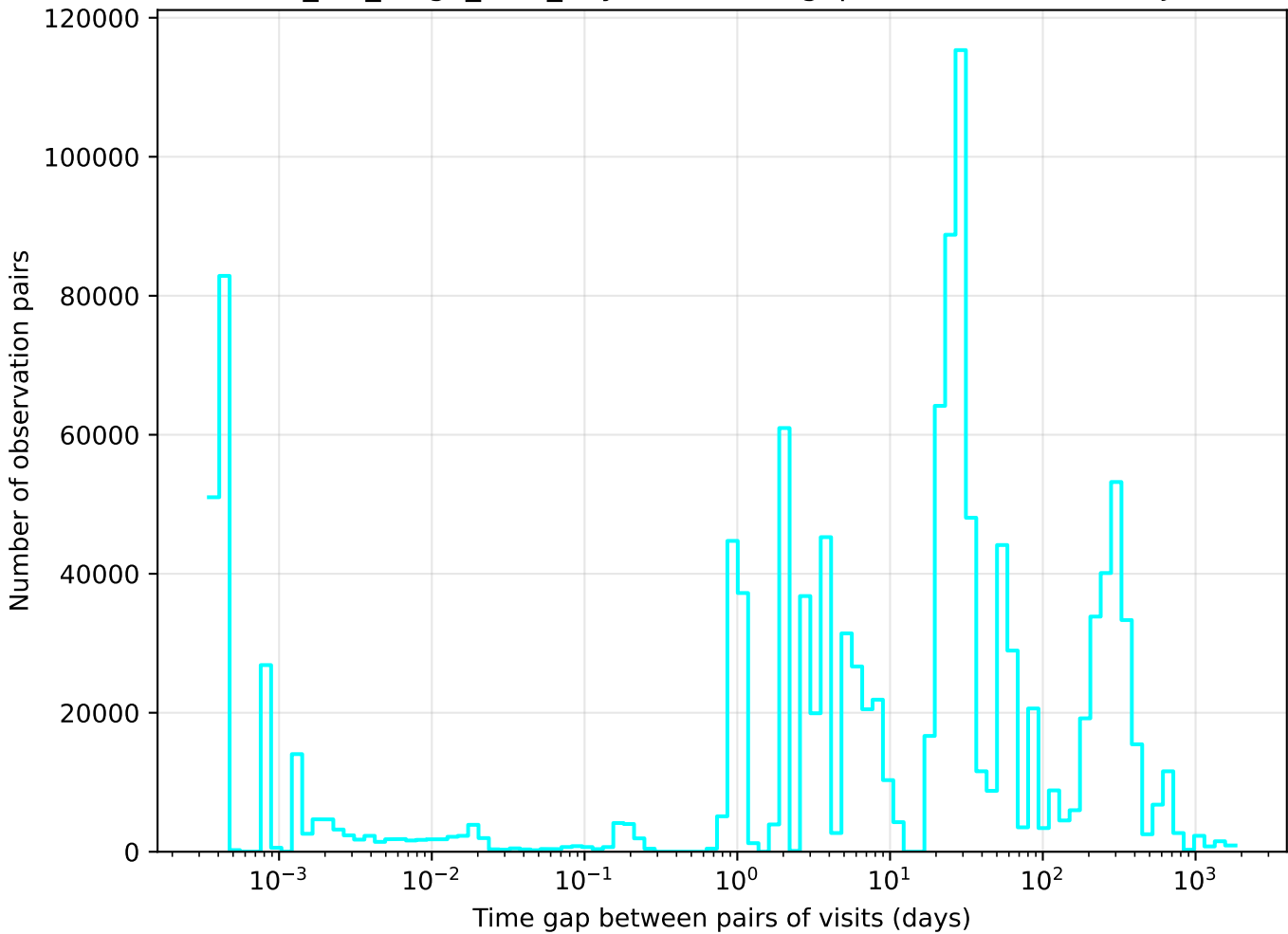
mw_roll_bulge_v3.3_10yrs u band: Tgaps observationStartMJD
