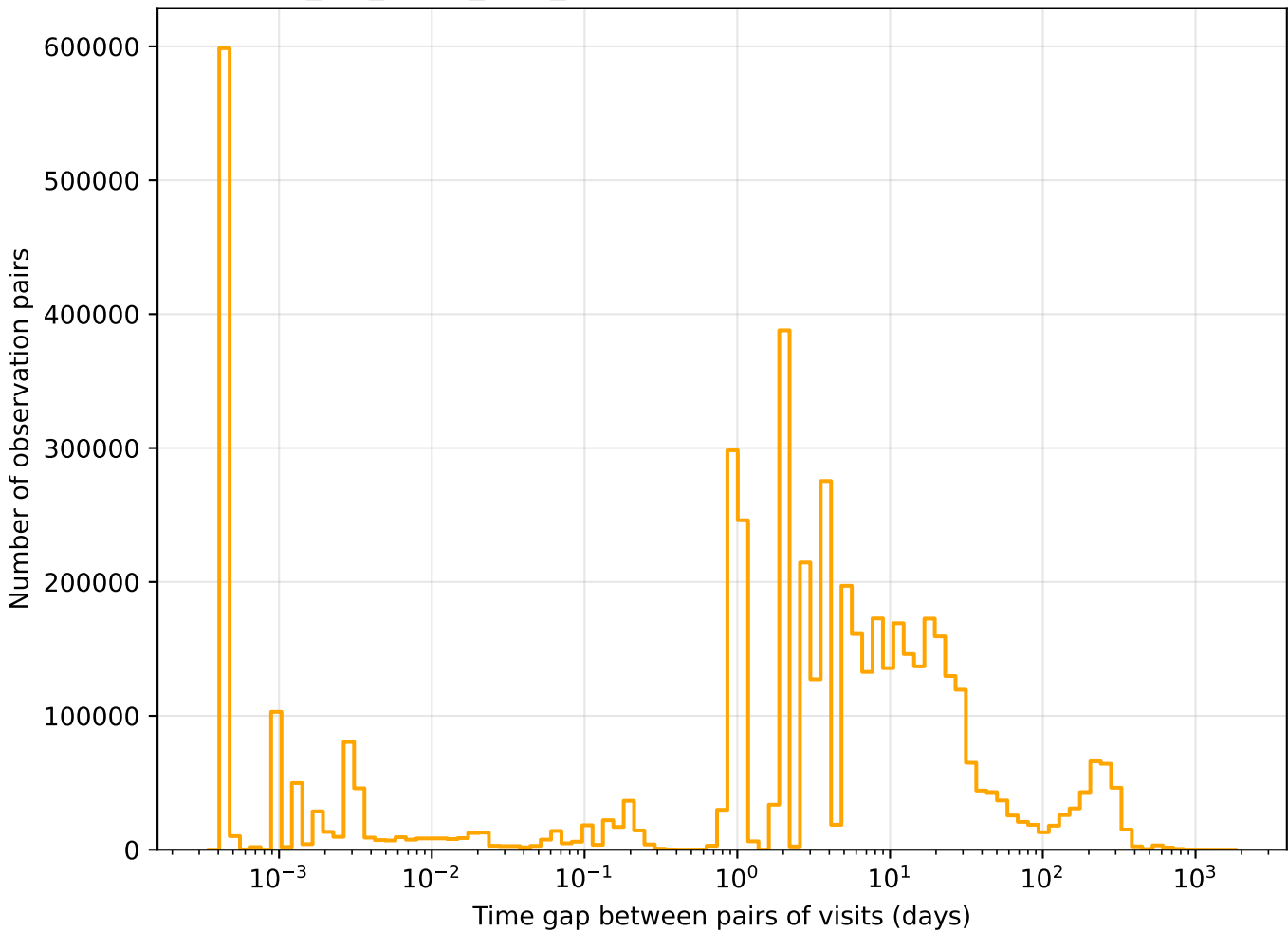
mw_roll_bulge_v3.3_10yrs r band: Tgaps observationStartMJD
