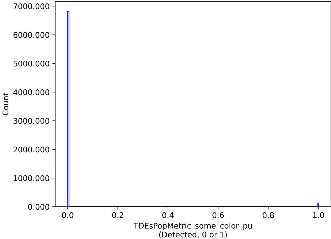
mw_roll_bulge_v3.3_10yrs : TDEsPopMetric_some_color_pu
