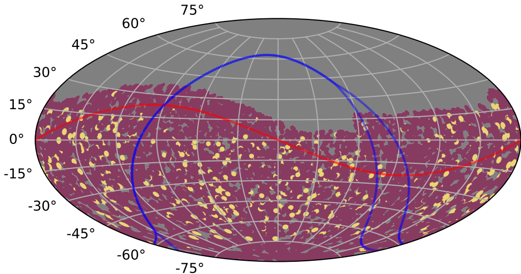
mw_roll_bulge_v3.3_10yrs : TDEsPopMetric_some_color
