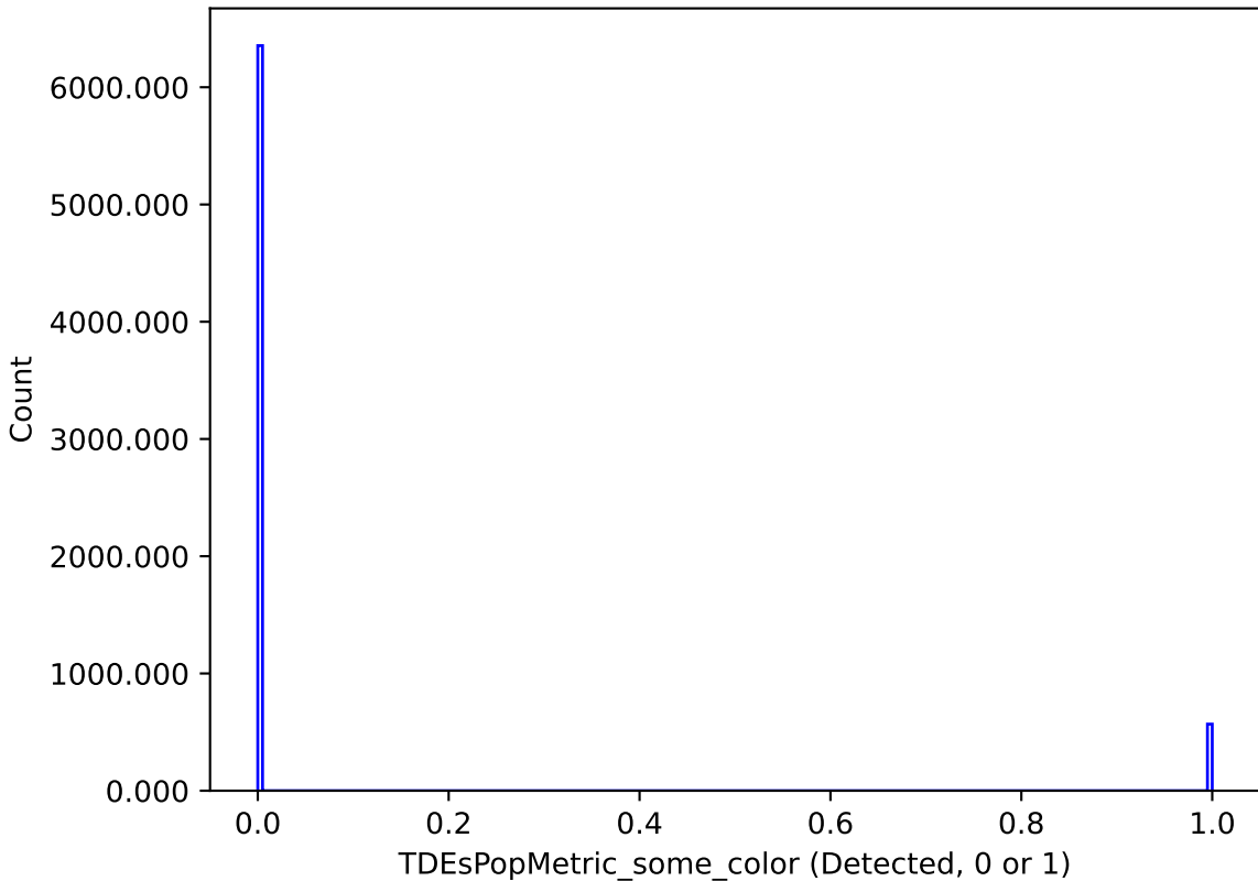
mw_roll_bulge_v3.3_10yrs : TDEsPopMetric_some_color
