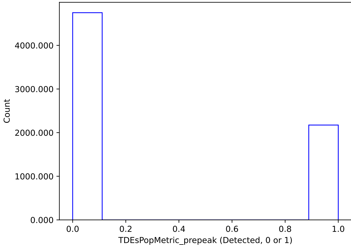
mw_roll_bulge_v3.3_10yrs : TDEsPopMetric_prepeak
