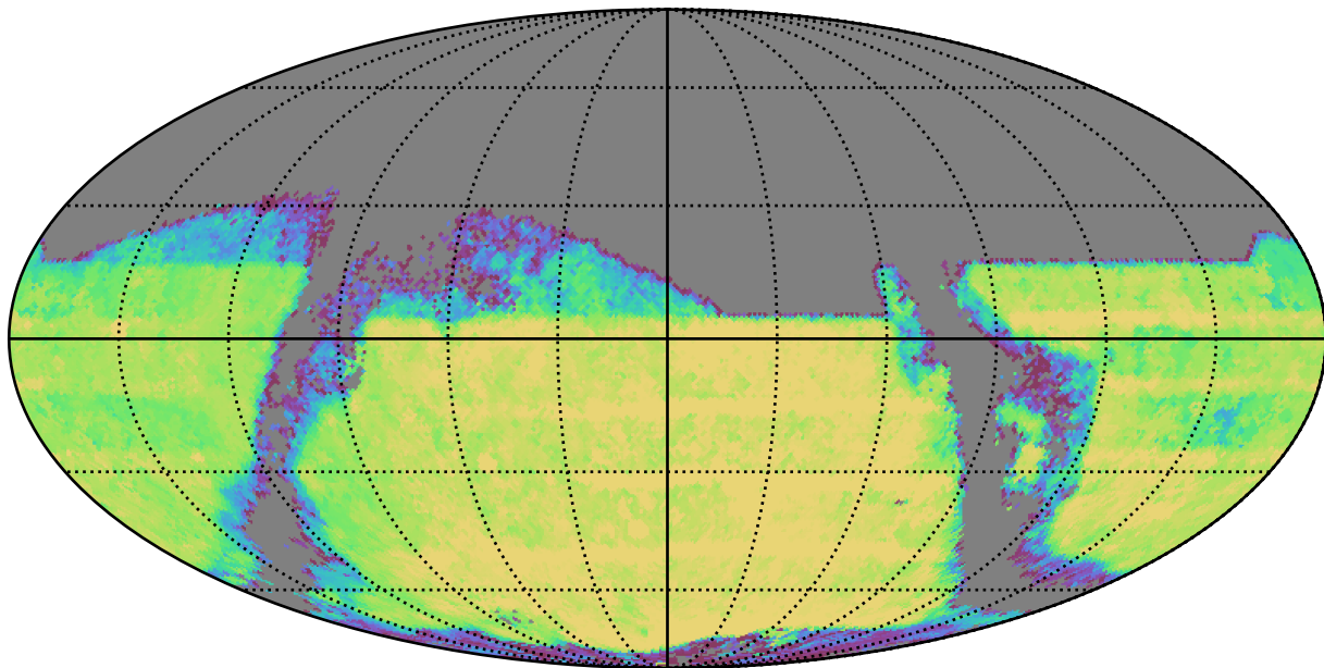
mw_roll_bulge_v3.3_10yrs : TDC_season
