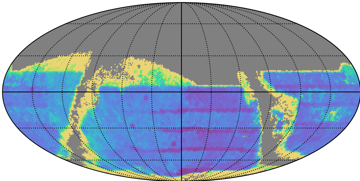
mw_roll_bulge_v3.3_10yrs : TDC_accuracy
