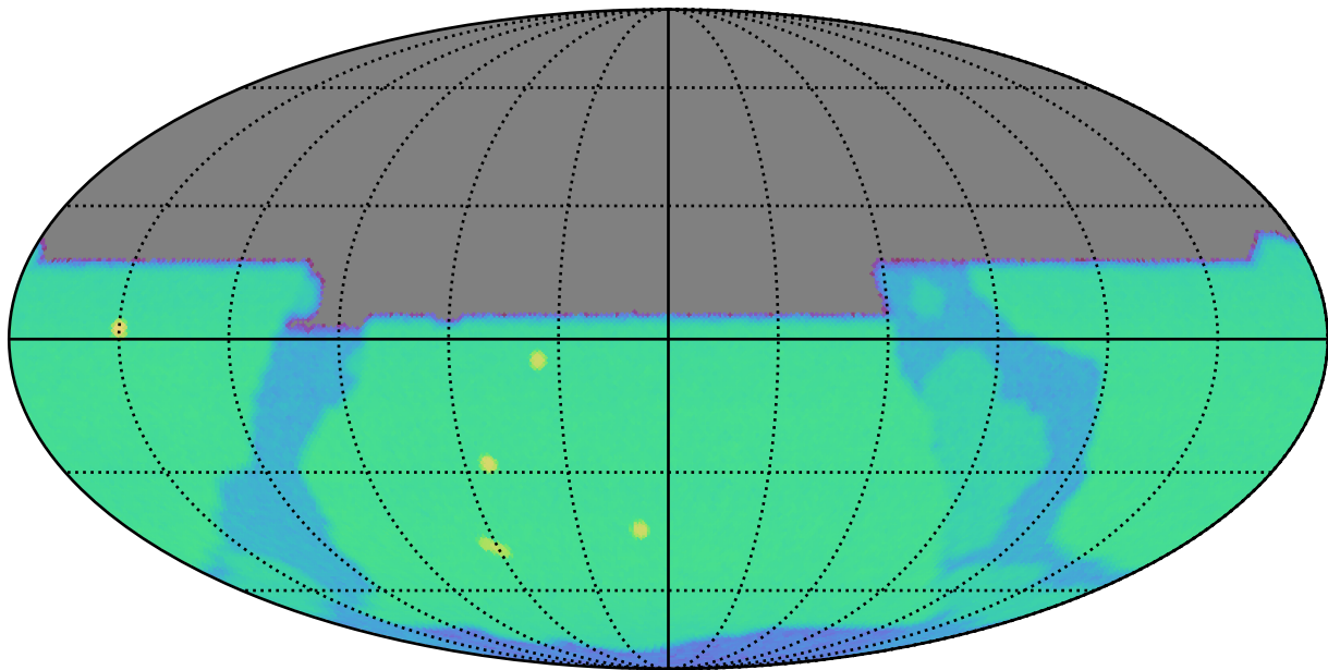
mw_roll_bulge_v3.3_10yrs y: SurfaceBrightLimit
