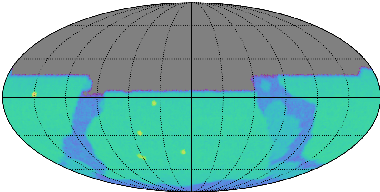
mw_roll_bulge_v3.3_10yrs u: SurfaceBrightLimit
