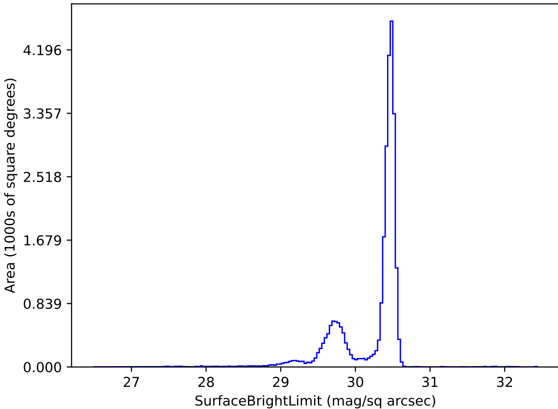
mw_roll_bulge_v3.3_10yrs r: SurfaceBrightLimit
