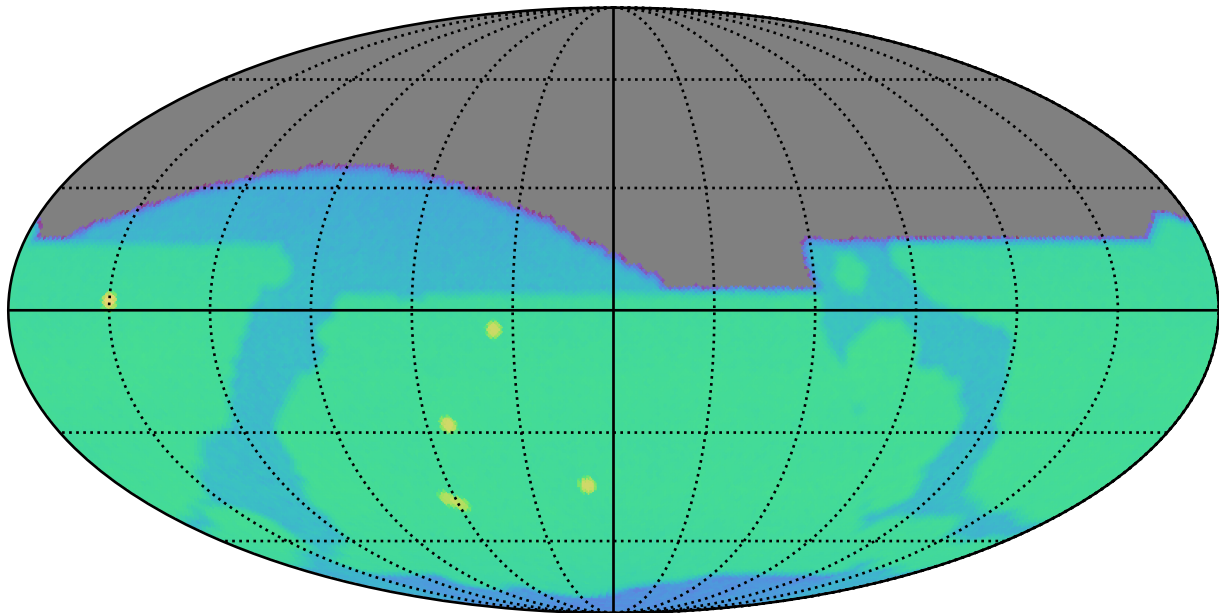
mw_roll_bulge_v3.3_10yrs i: SurfaceBrightLimit
