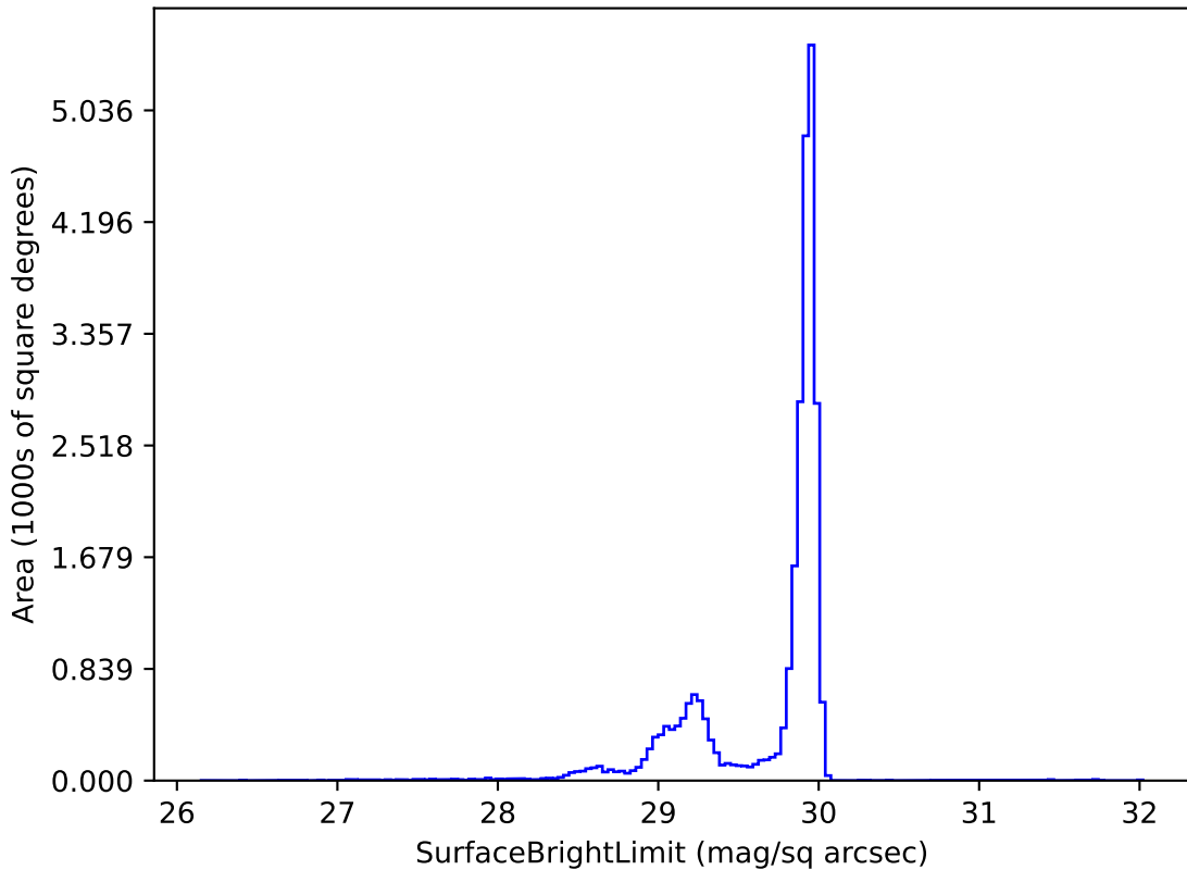
mw_roll_bulge_v3.3_10yrs i: SurfaceBrightLimit
