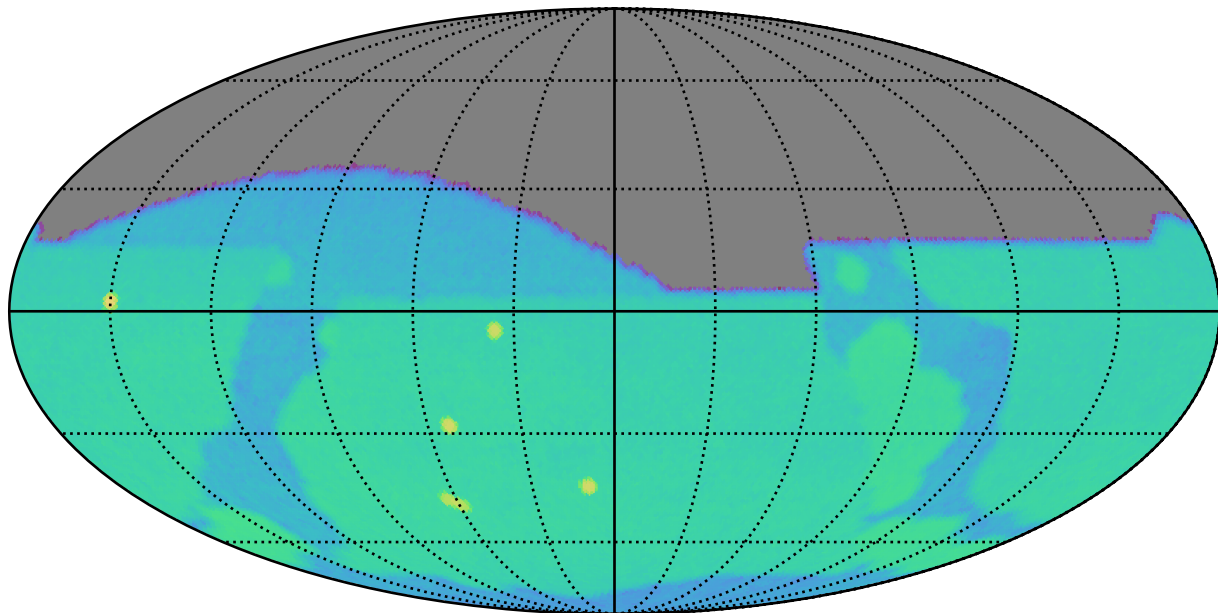
mw_roll_bulge_v3.3_10yrs g: SurfaceBrightLimit
