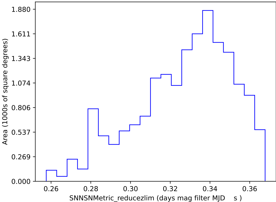
mw_roll_bulge_v3.3_10yrs DDF excluded: SNNSNMetric_reducezlim
