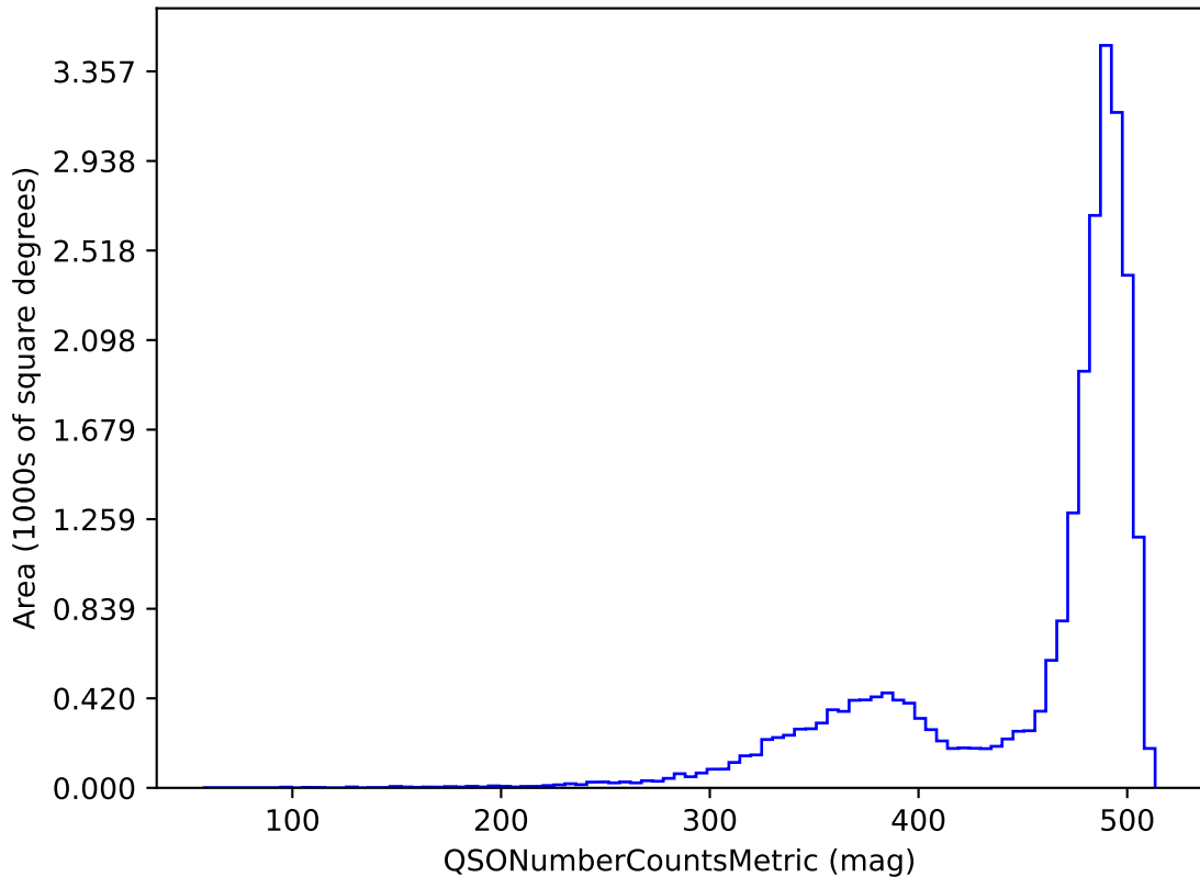
mw_roll_bulge_v3.3_10yrs z band and non-DD: QSONumberCountsMetric
