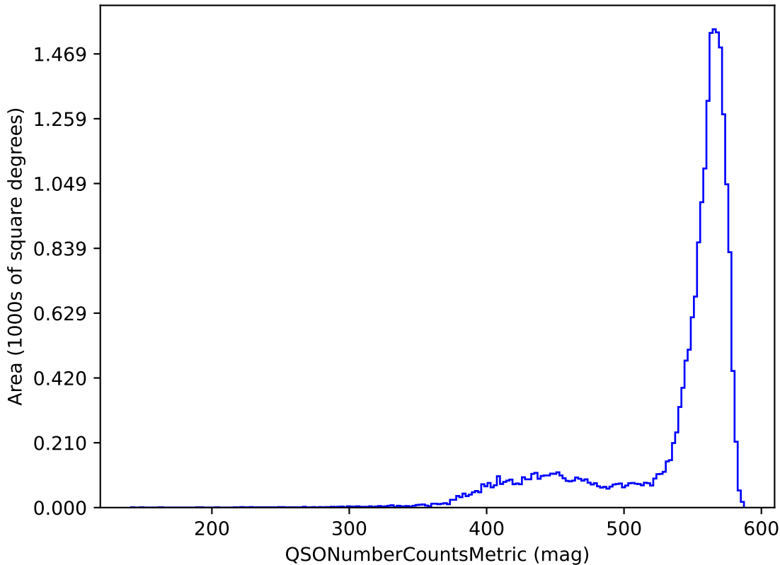
mw_roll_bulge_v3.3_10yrs y band and non-DD: QSONumberCountsMetric
