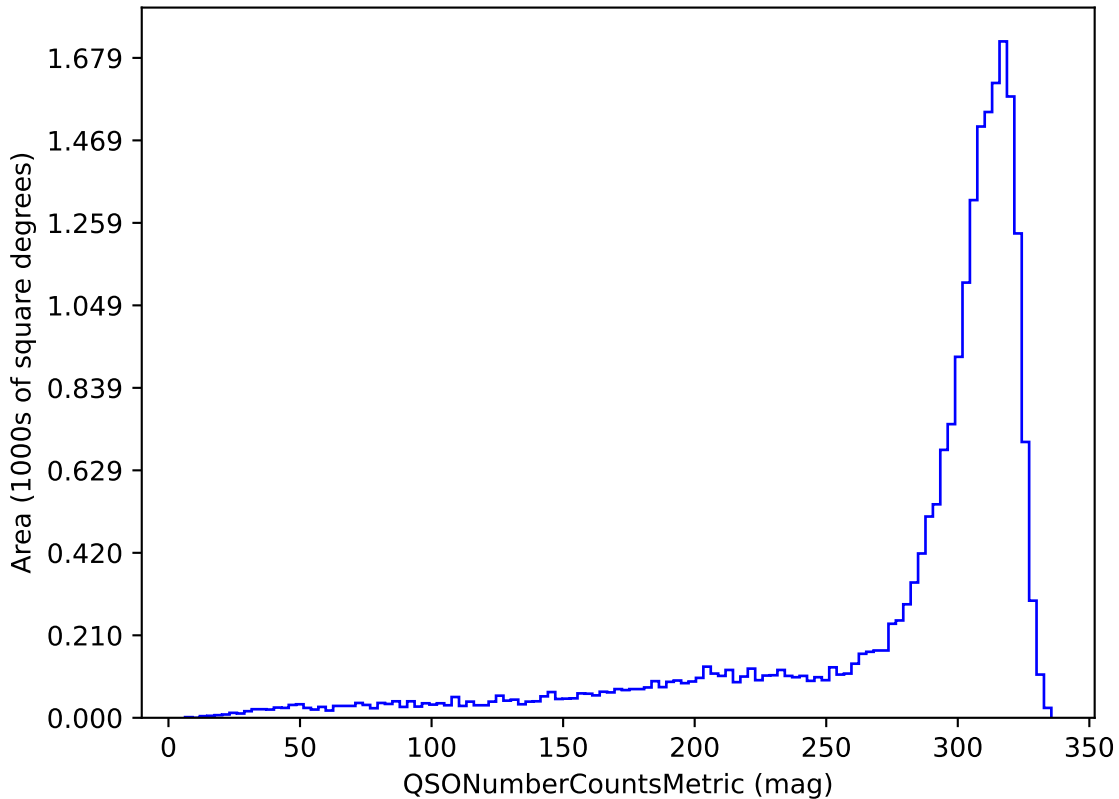
mw_roll_bulge_v3.3_10yrs u band and non-DD: QSONumberCountsMetric
