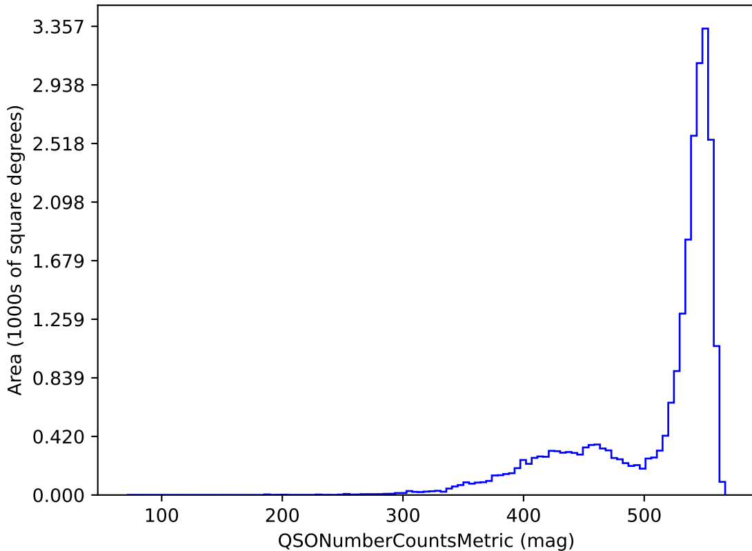
mw_roll_bulge_v3.3_10yrs i band and non-DD: QSONumberCountsMetric
