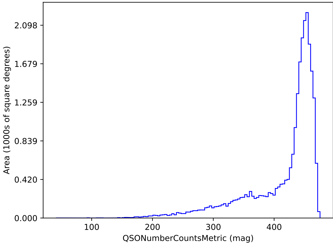
mw_roll_bulge_v3.3_10yrs g band and non-DD: QSONumberCountsMetric
