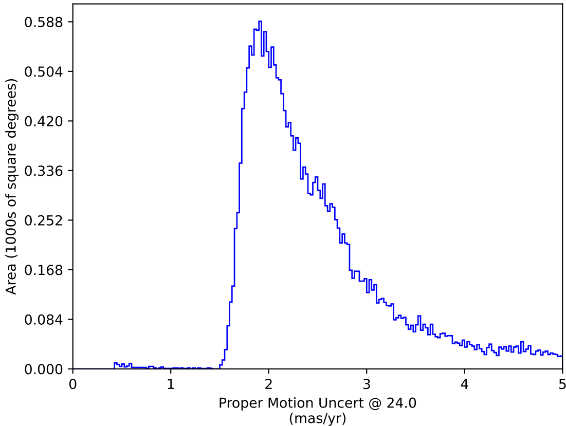
mw_roll_bulge_v3.3_10yrs : Proper Motion Uncert @ 24.0
