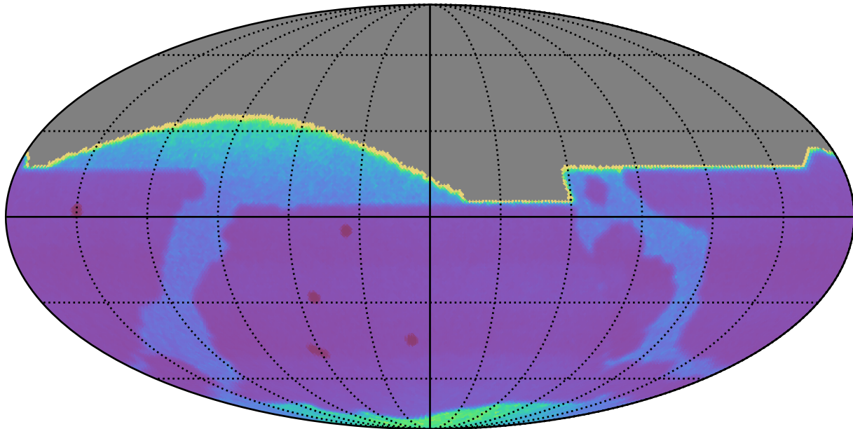
mw_roll_bulge_v3.3_10yrs : Proper Motion Uncert @ 20.5
