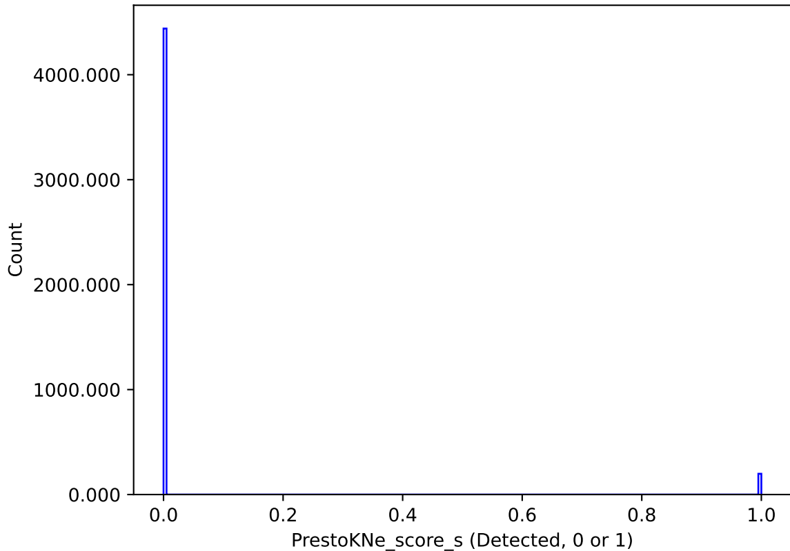
mw_roll_bulge_v3.3_10yrs : PrestoKNe_score_s
