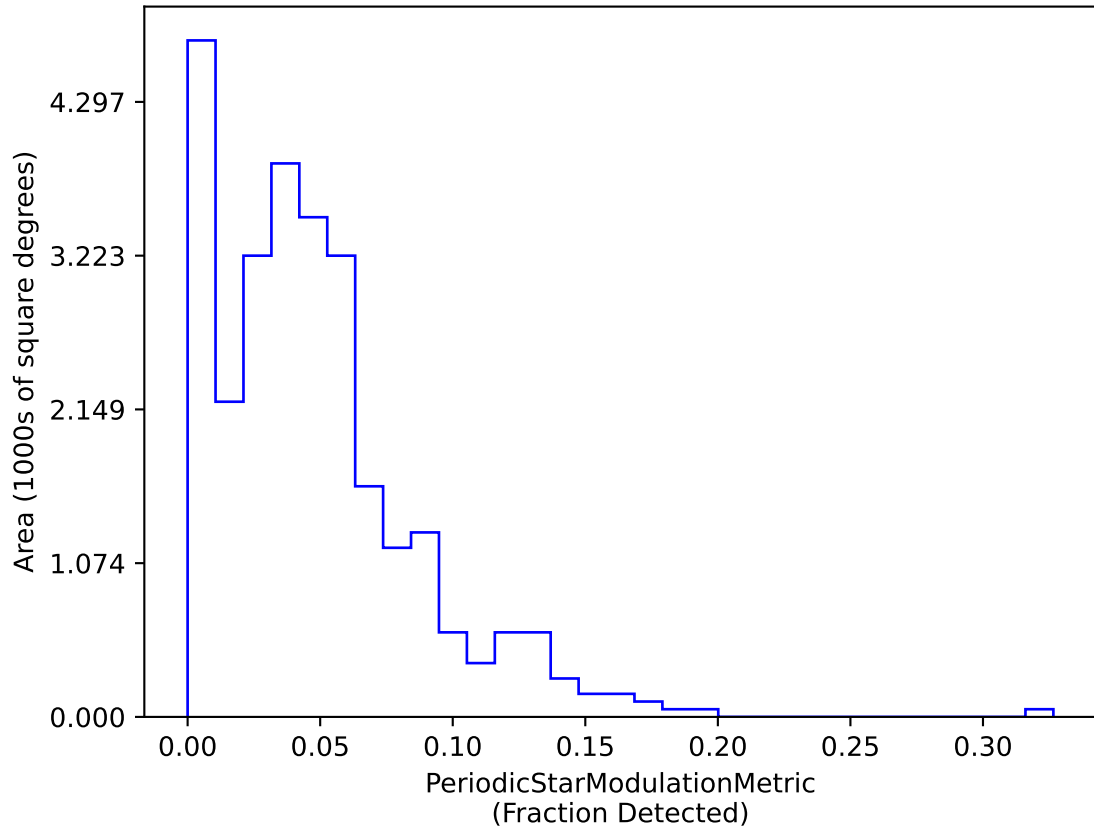
mw_roll_bulge_v3.3_10yrs dm 20 interval 15 RRC Year 1-2: PeriodicStarModulationMetric
