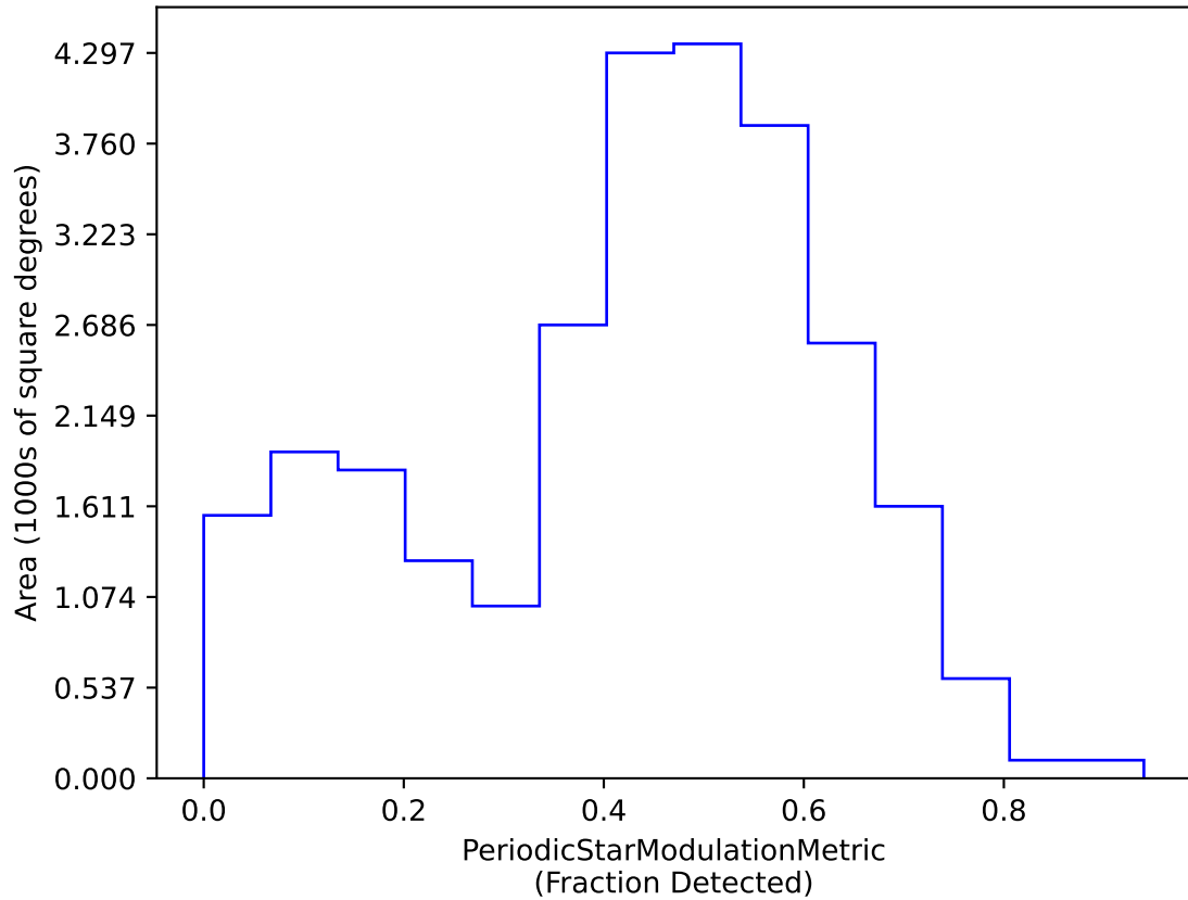
mw_roll_bulge_v3.3_10yrs dm 18 interval 30 RRC Year 1-2: PeriodicStarModulationMetric
