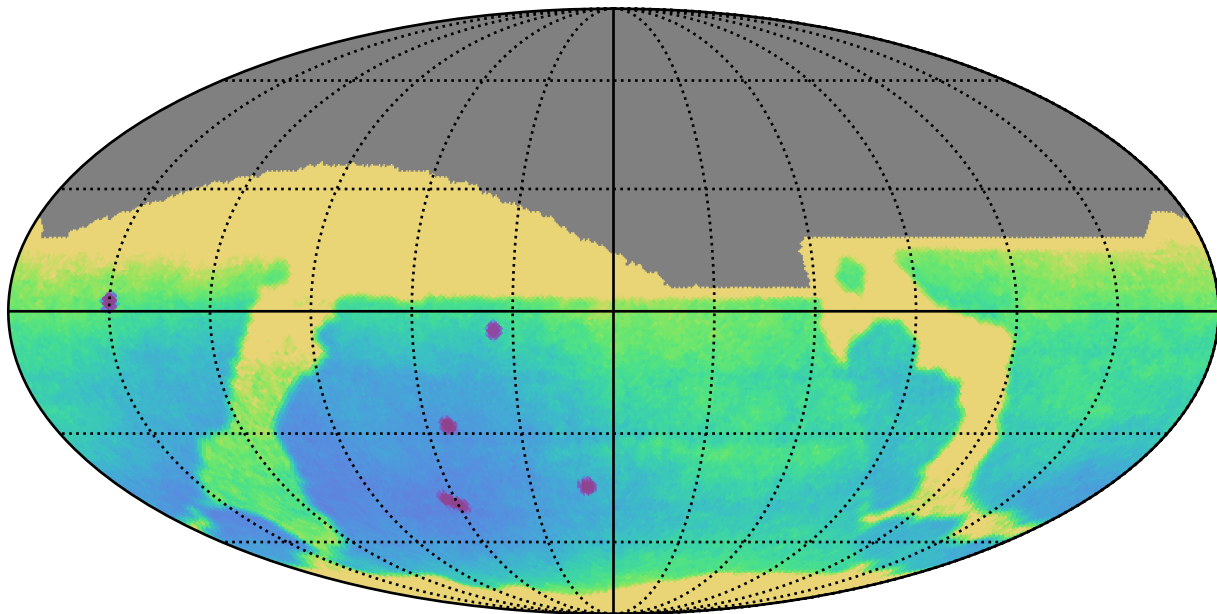
mw_roll_bulge_v3.3_10yrs : Parallax Uncert @ 24.0
