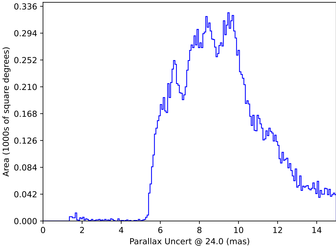
mw_roll_bulge_v3.3_10yrs : Parallax Uncert @ 24.0
