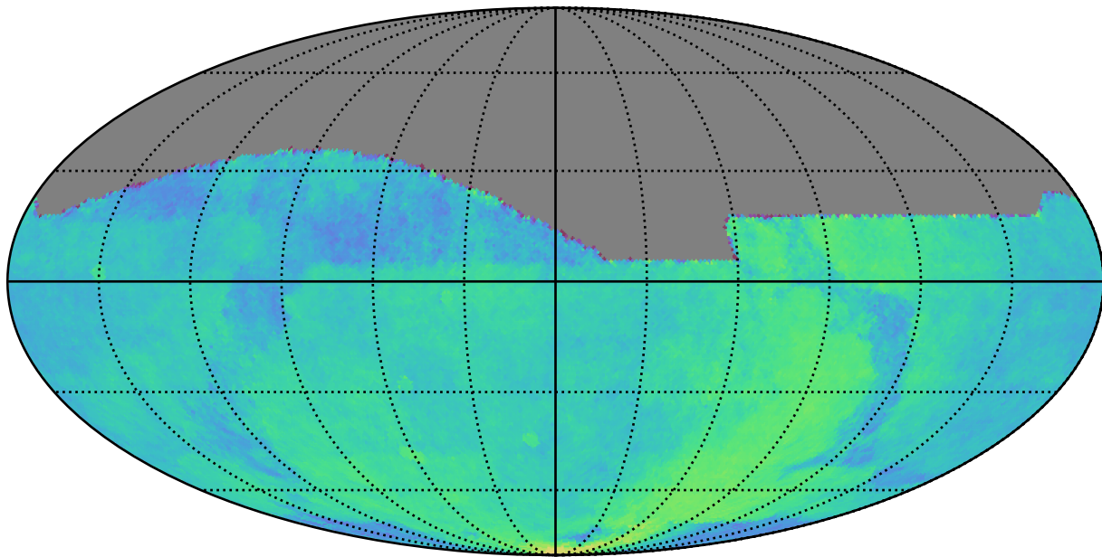
mw_roll_bulge_v3.3_10yrs : Parallax Coverage @ 24.0
