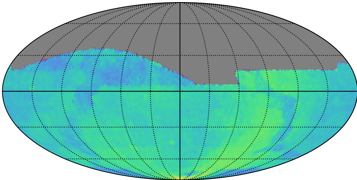
mw_roll_bulge_v3.3_10yrs : Parallax Coverage @ 22.4
