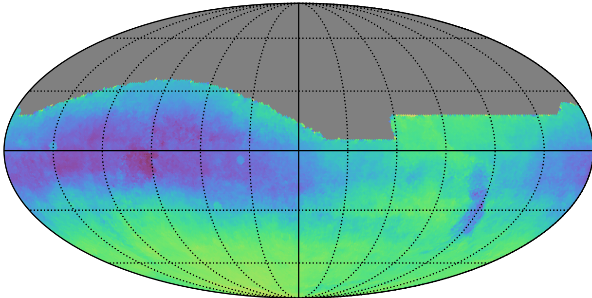
mw_roll_bulge_v3.3_10yrs : Parallax-DCR degeneracy @ 24.0
