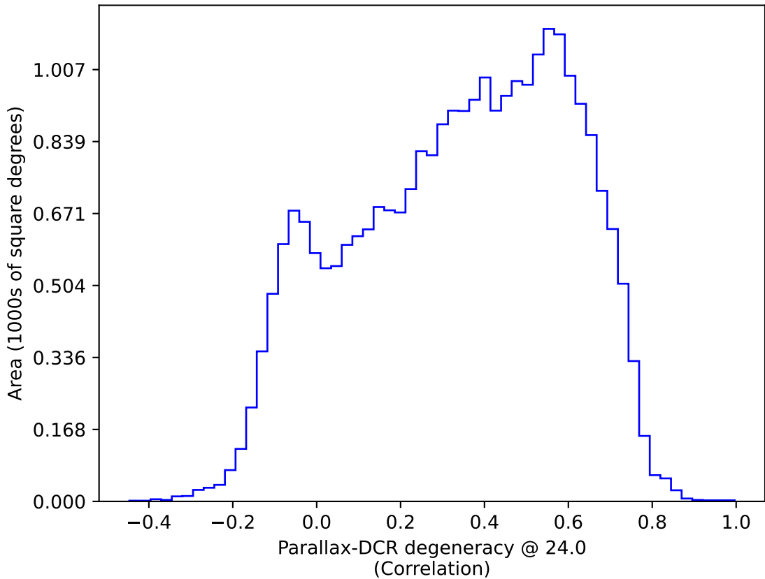
mw_roll_bulge_v3.3_10yrs : Parallax-DCR degeneracy @ 24.0
