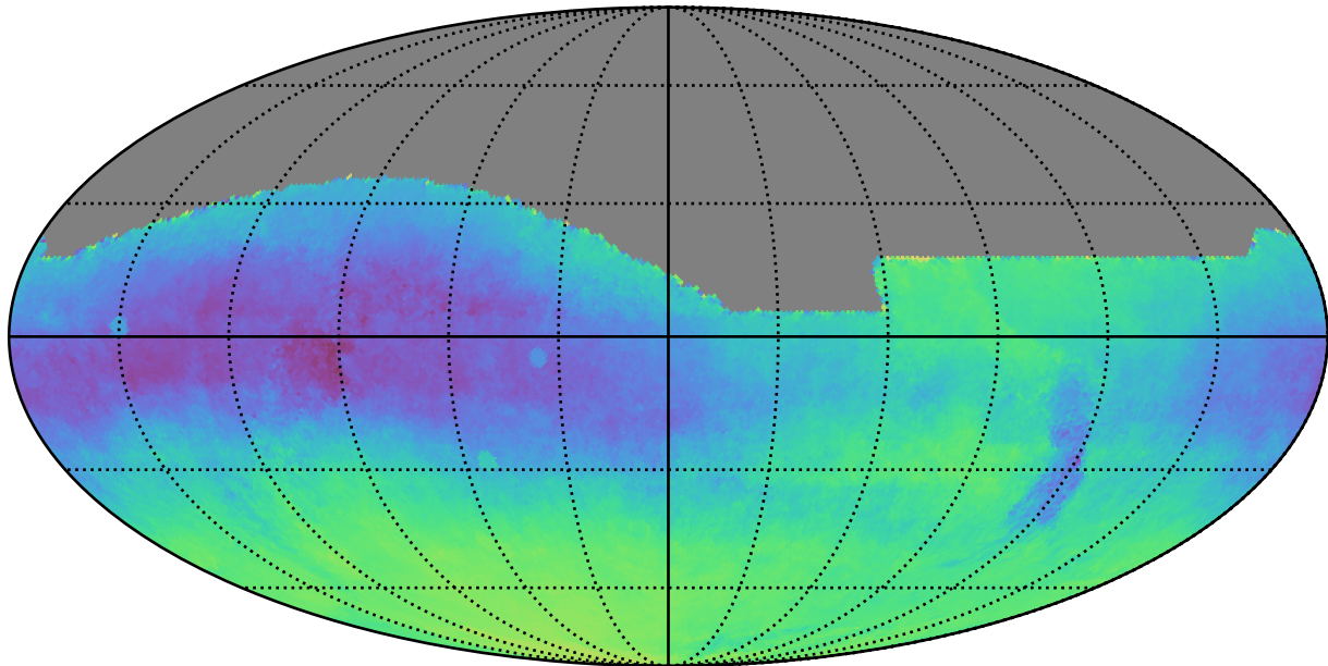
mw_roll_bulge_v3.3_10yrs : Parallax-DCR degeneracy @ 22.4
