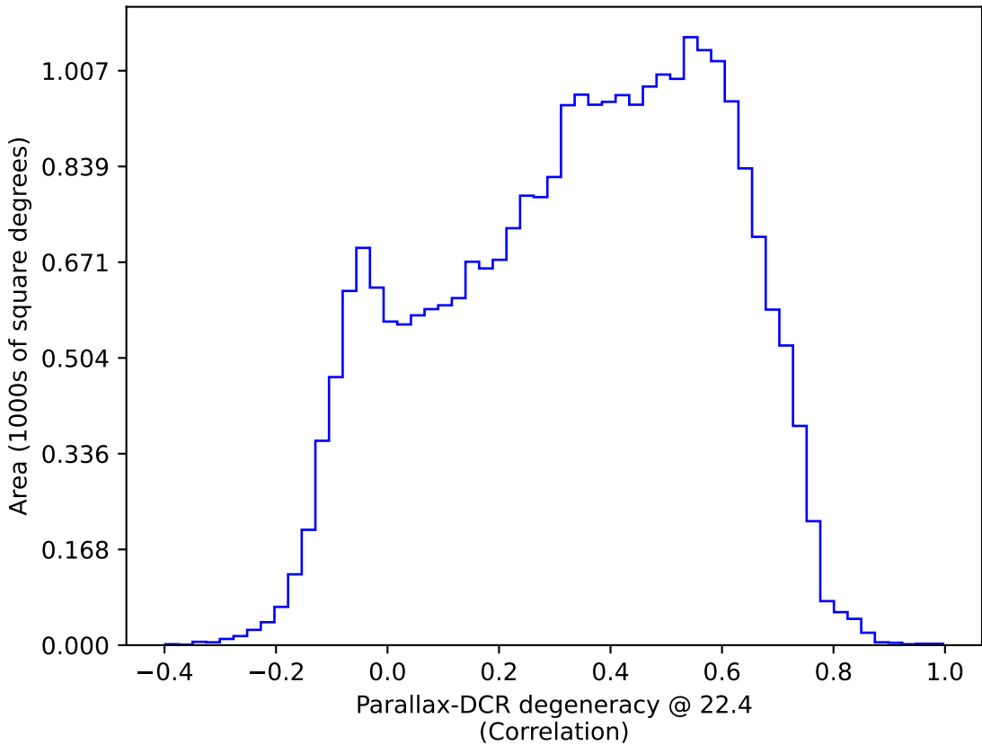
mw_roll_bulge_v3.3_10yrs : Parallax-DCR degeneracy @ 22.4
