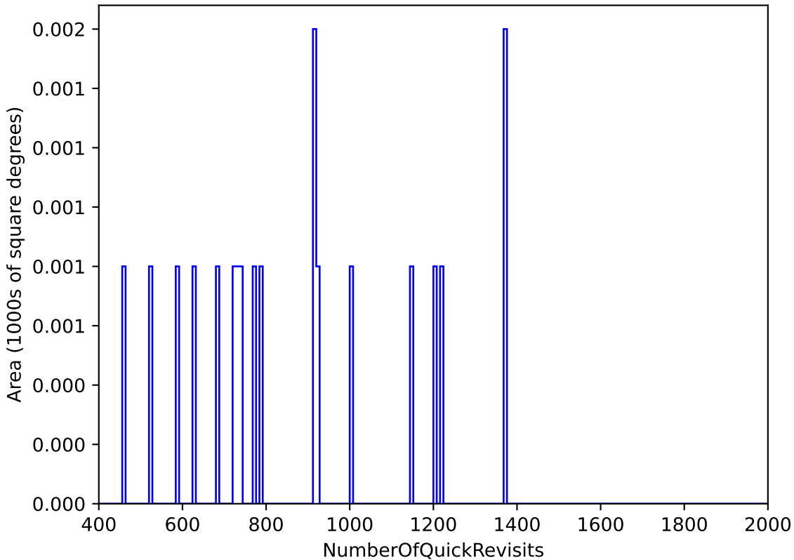
mw_roll_bulge_v3.3_10yrs : NumberOfQuickRevisits
