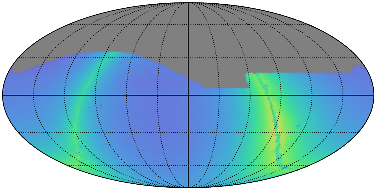
mw_roll_bulge_v3.3_10yrs z: Nstars_no_crowding
