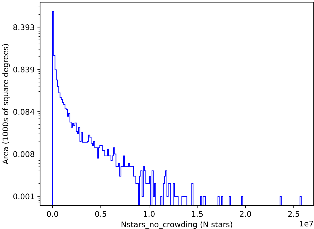
mw_roll_bulge_v3.3_10yrs y: Nstars_no_crowding
