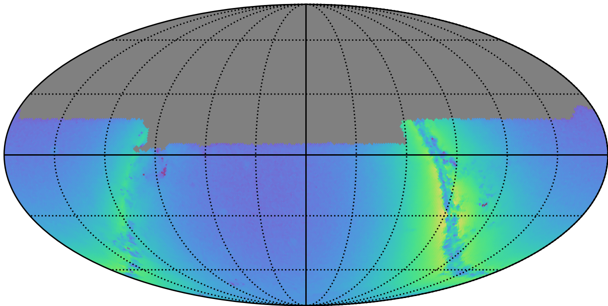
mw_roll_bulge_v3.3_10yrs u: Nstars_no_crowding
