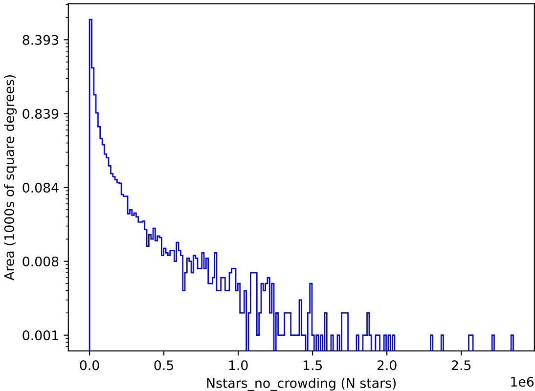
mw_roll_bulge_v3.3_10yrs u: Nstars_no_crowding
