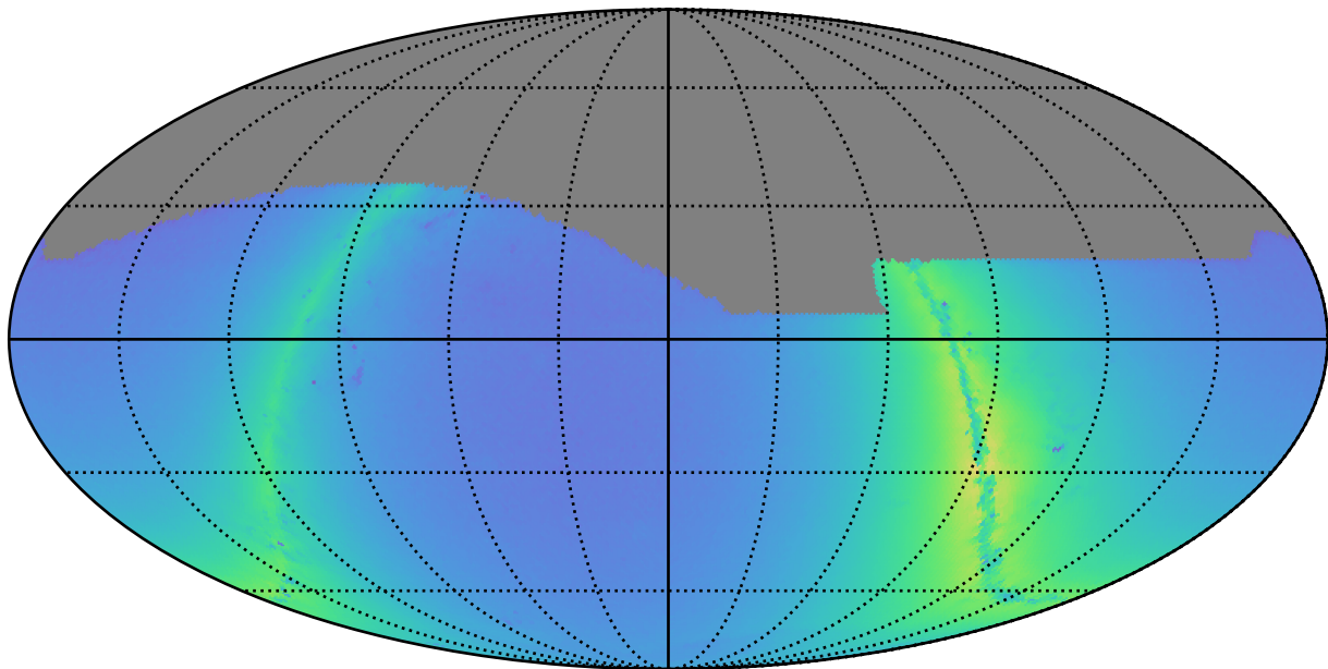
mw_roll_bulge_v3.3_10yrs r: Nstars_no_crowding
